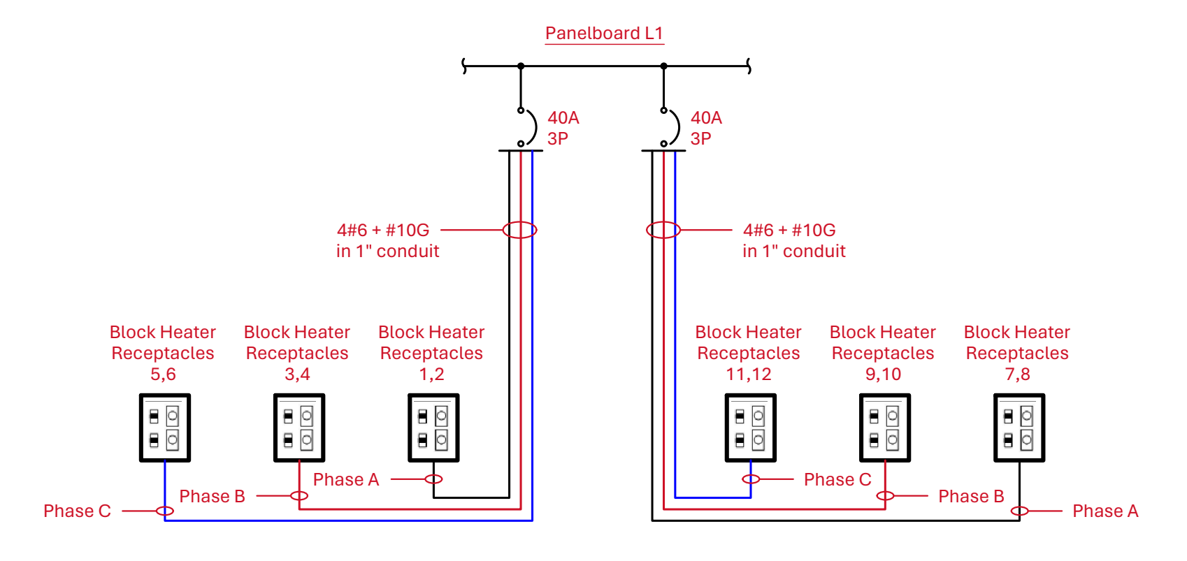
2 Block Heater Recept Wiring Diagram Scale: Not Drawn to Scale
